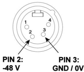
DPS-48 Male connectors pinout
