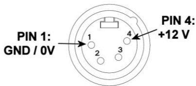
DPS-12 Male connectors pinout
